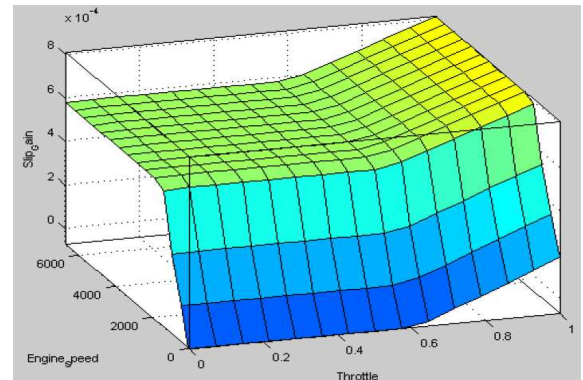
Fig. 6. Fuzzy logic surface throttle against engine speed
