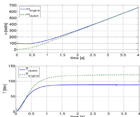
Fig. 14. Clutch engagement and transmission torque
