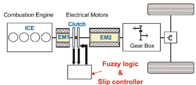
Fig. 1. Configuration of parallel hybrid powertrain
