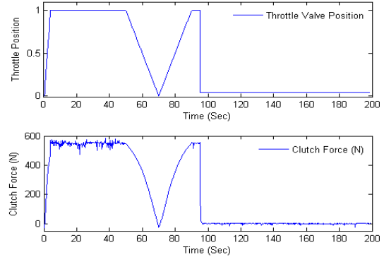
Fig. 11. Performance of automatic clutch controller
