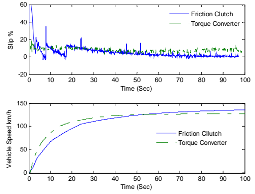
Fig. 10. Clutch slip and vehicle speed
