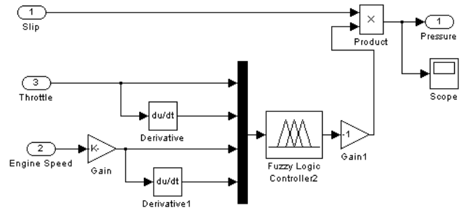
Fig. 4. Fuzzy friction clutch controller
