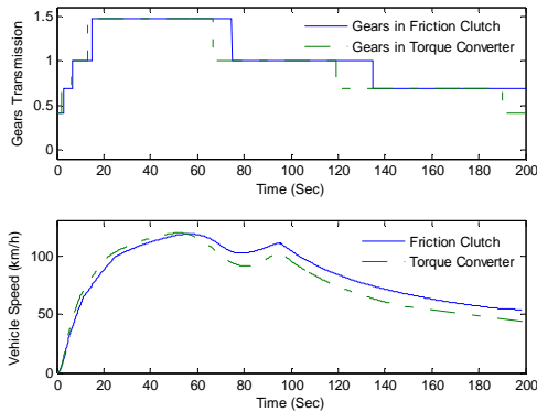
Fig. 9. Automatic gear shifting and vehicle speed
