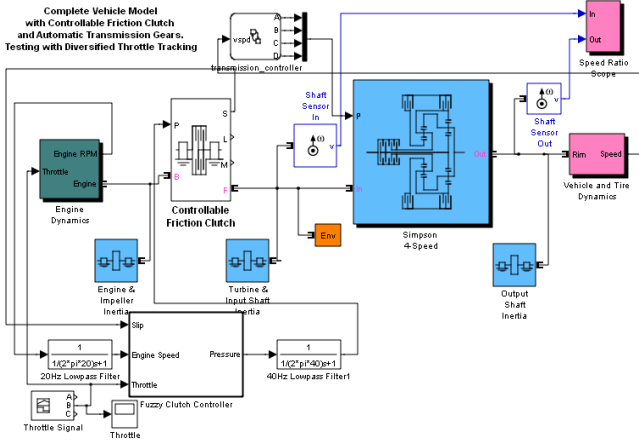
Fig. 8. Comprehensive simulation
