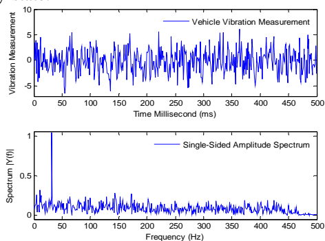
Fig. 12. Amplitude Spectrum of Vehicle Noise Measurement
