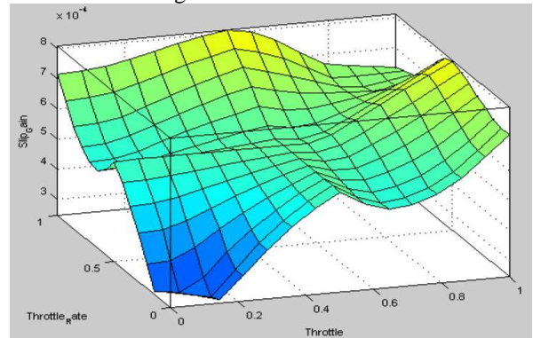
Fig. 5. Fuzzy logic surface throttle against throttle rate
