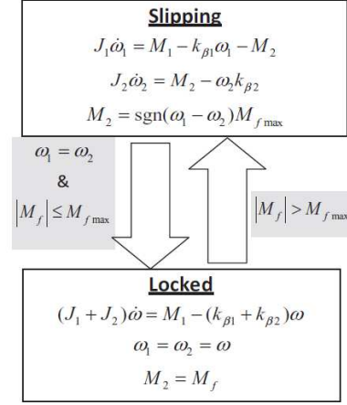
Fig. 3. Friction mode transmissions
