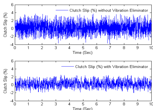
Fig. 16. Performance of clutch with vibration eliminators
