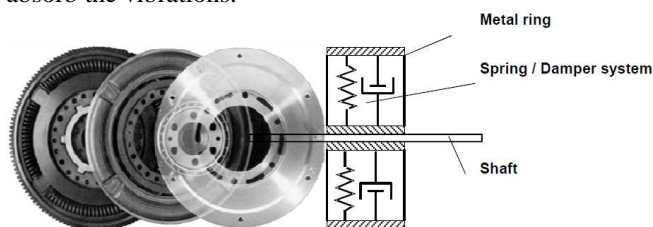
Fig. 15. Clutch with vibration eliminators
